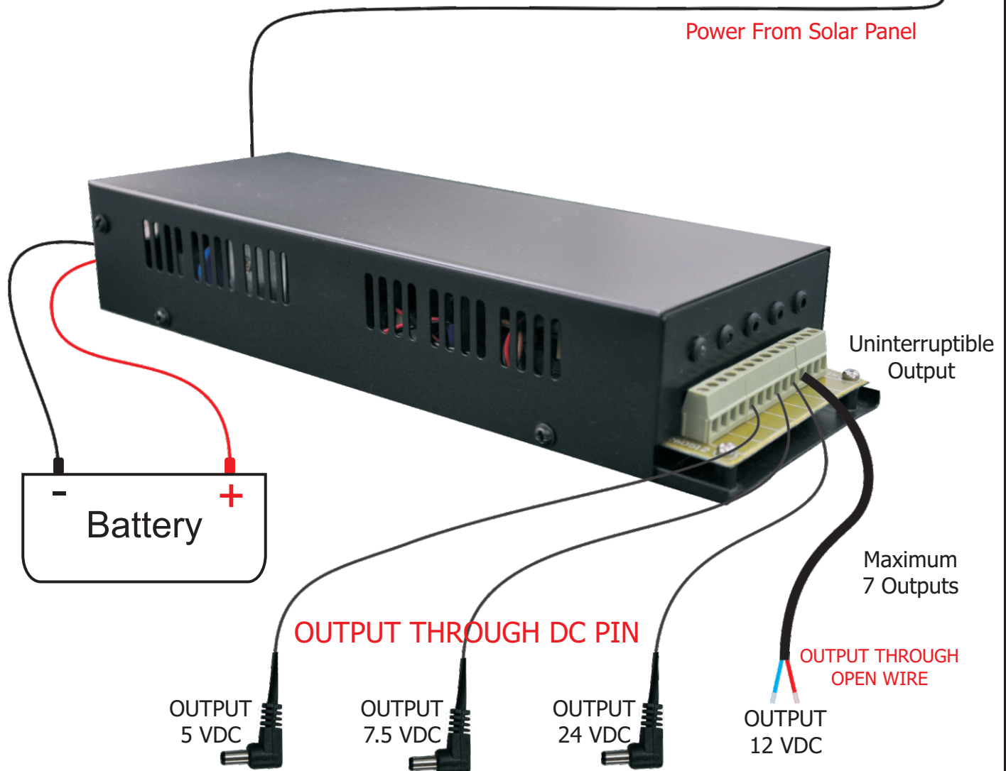
SOLAR PANEL
